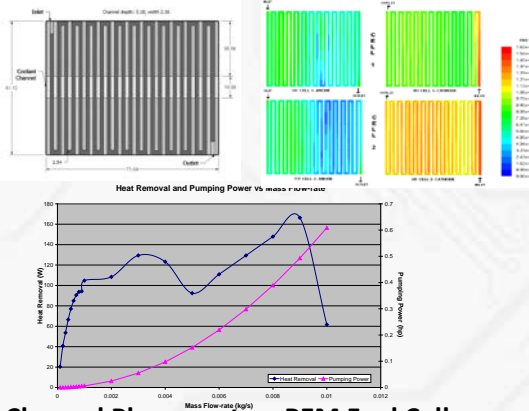
Effect of Optimal Coolant Channel Placement on PEM Fuel Cell Performance
