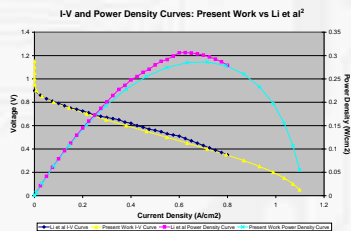
Effect of Optimal Coolant Channel Placement on PEM Fuel Cell Performance
